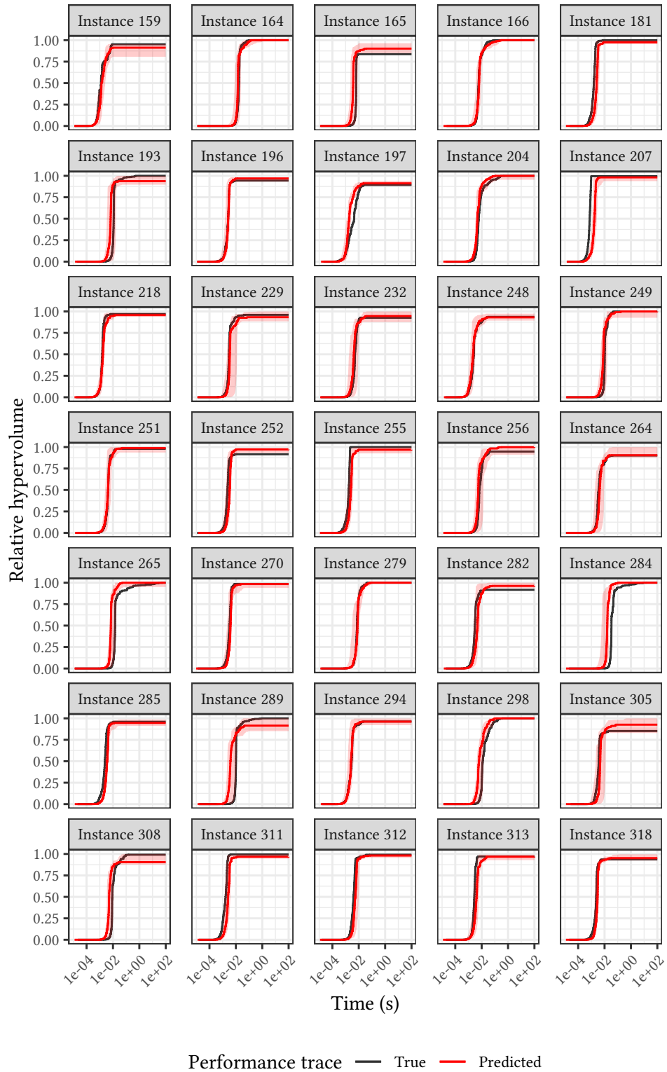
Figure A.5: Results of anytime performance prediction on the testing data set.
