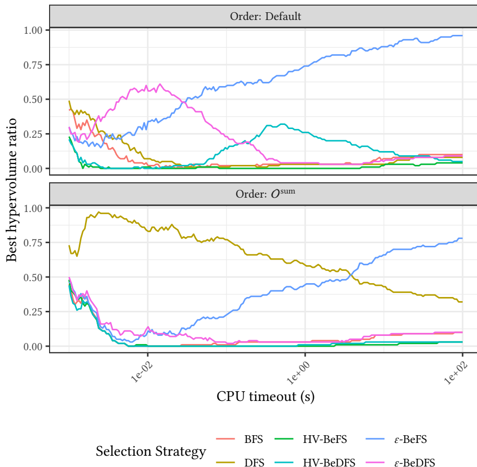
Figure 6.8: Ratio of test scenarios, with 7 objectives and a given CPU timeout value, for which a selection strategy found the best archive with respect to the hypervolume quality indicator.
