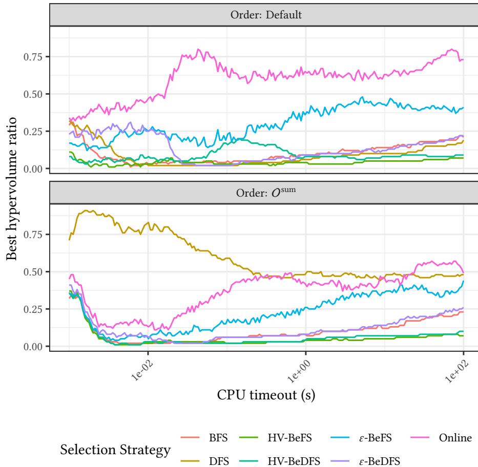
Figure 6.14: Ratio of test scenarios, with 5 objectives and a given CPU timeout value, for which a selection strategy found the best archive with respect to the hypervolume quality indicator.
