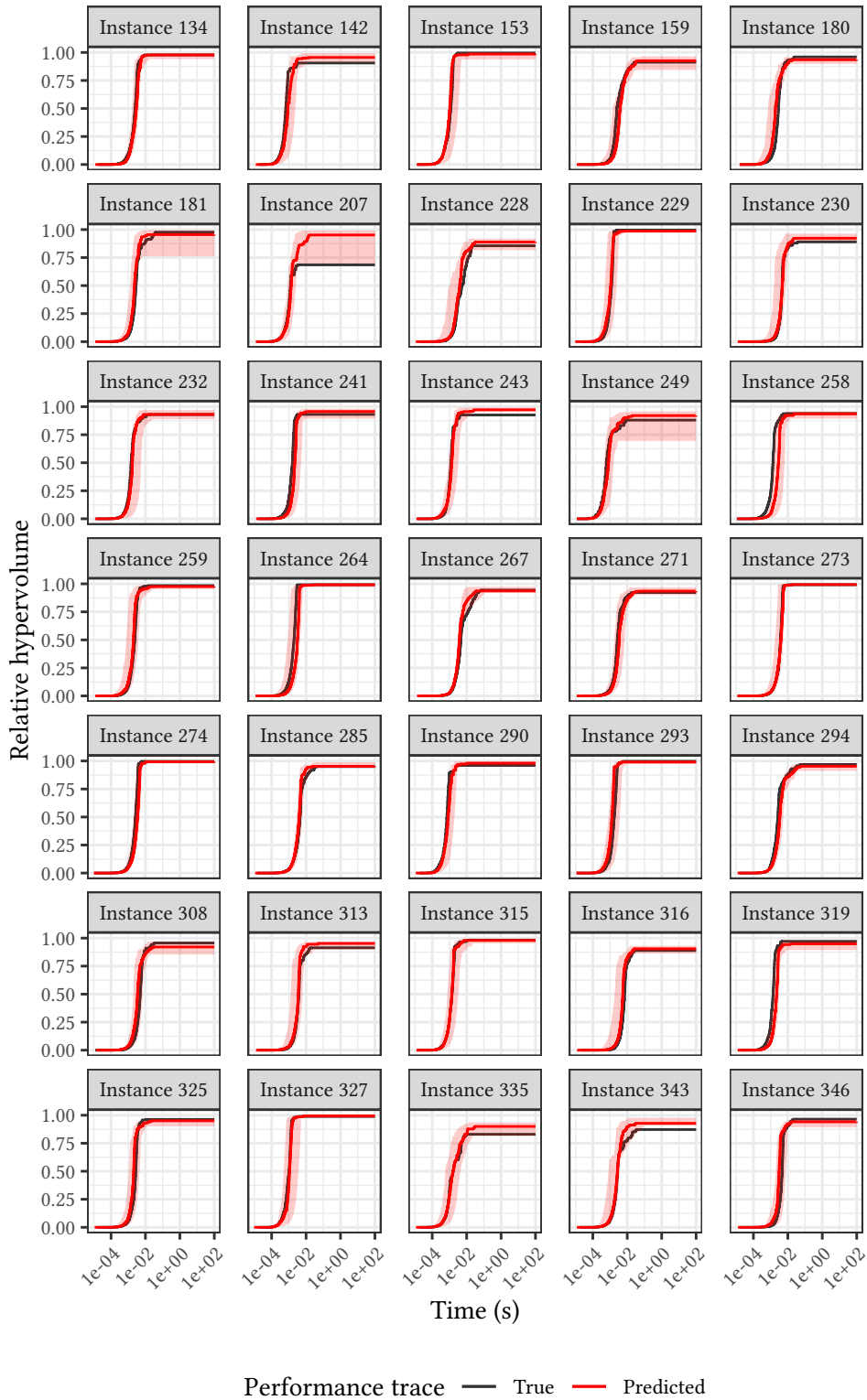
Figure A.2: Results of anytime performance prediction on the testing data set.
