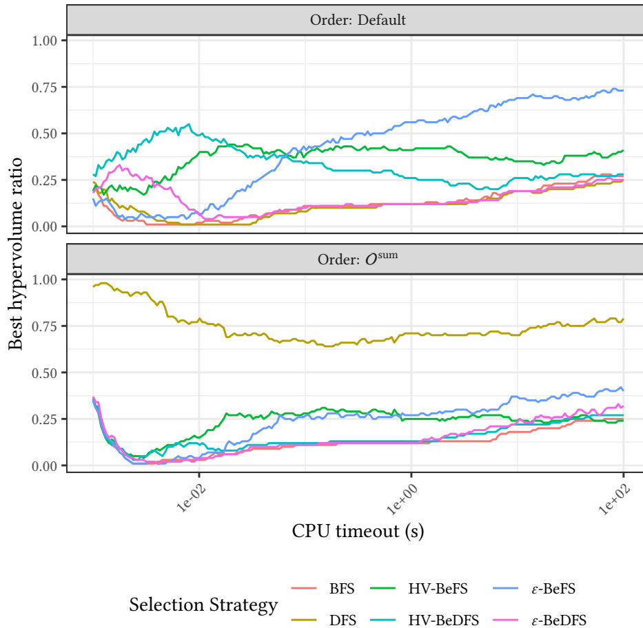
Figure 6.4: Ratio of test scenarios, with 3 objectives and a given CPU timeout value, for which a selection strategy found the best archive with respect to the hypervolume quality indicator.
