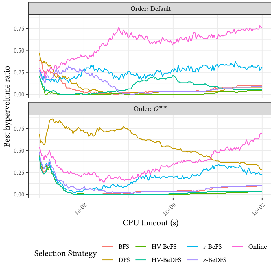
Figure 6.16: Ratio of test scenarios, with 7 objectives and a given CPU timeout value, for which a selection strategy found the best archive with respect to the hypervolume quality indicator.
