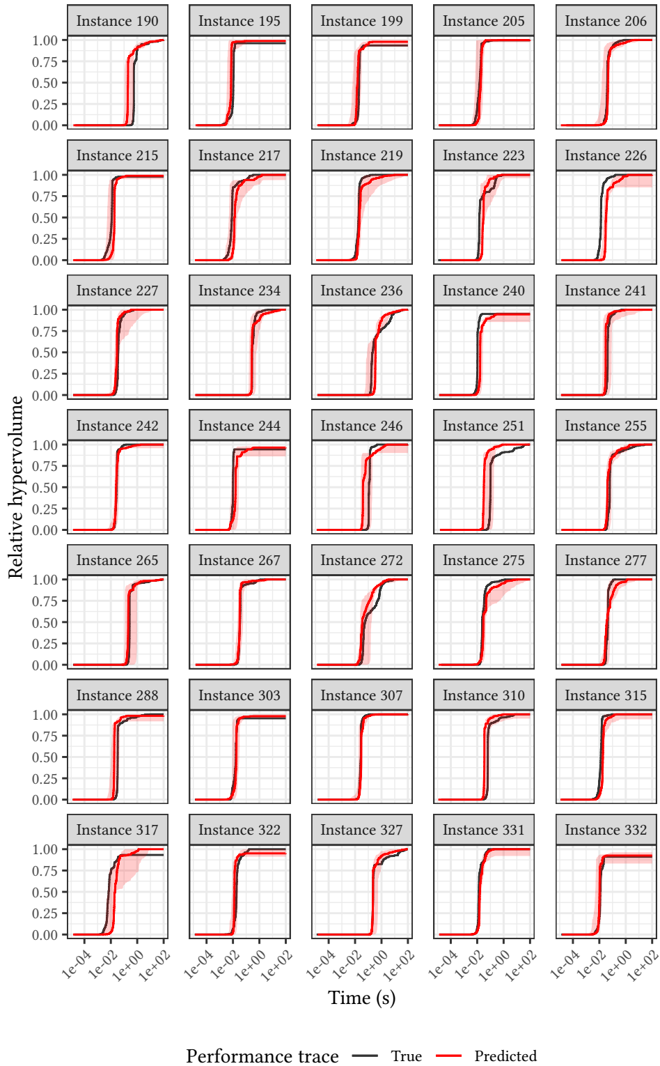
Figure A.8: Results of anytime performance prediction on the testing data set.
