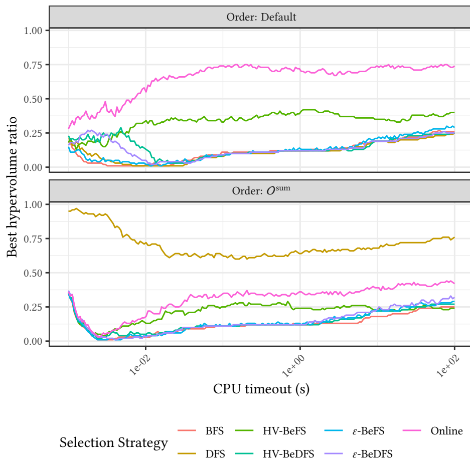
Figure 6.12: Ratio of test scenarios, with 3 objectives and a given CPU timeout value, for which a selection strategy found the best archive with respect to the hypervolume quality indicator.
