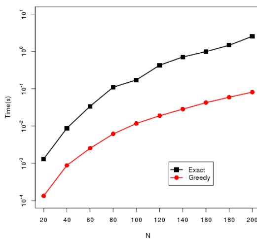
FIGURE 7.2: Time comparison for a varying n , k = 0.3n , correlation = 0
