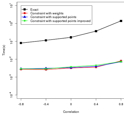
FIGURE 8.11: Time comparison for varying correlation, n = 100 , k = 0.3n
