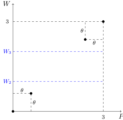
FIGURE 4.2: Illustration of the proof for Proposition 1
