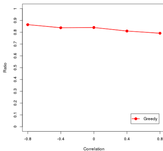
FIGURE 8.6: Error comparison for a varying correlation, n = 100 , k = 0.3n
