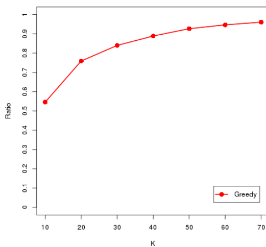
FIGURE 8.4: Error comparison for a varying k , n = 100 , correlation = 0
