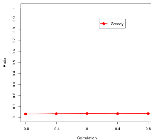
FIGURE 7.6: Error comparison for a varying correlation, N = 160 , k = 0.3n
