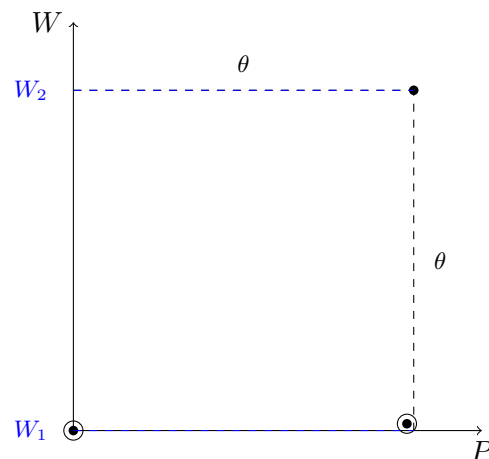
FIGURE 8.8: Illustration of the proof for Proposition 5 with set Y_* circled.
