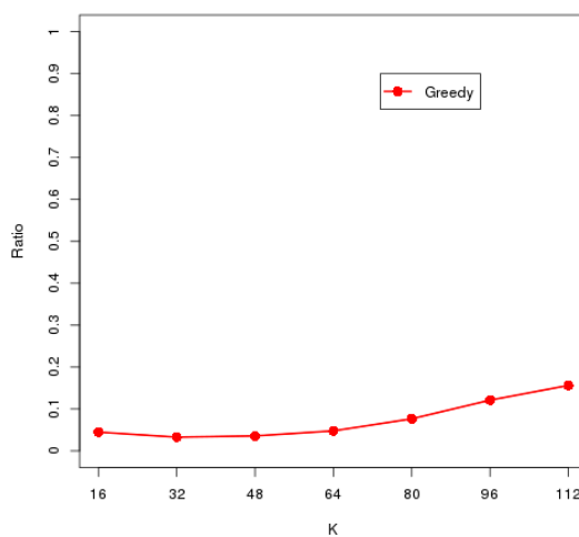
FIGURE 7.4: Error comparison for a varying k , n = 160 , correlation = 0
