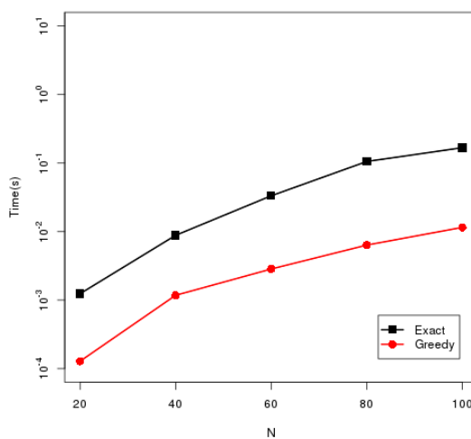
FIGURE 8.2: Time comparison for a varying n , k = 0.3n , correlation = 0
