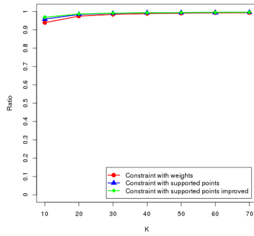
FIGURE 8.12: Error comparison for a varying k , n = 100 , correlation = 0
